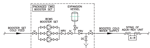
Installation Of Aqua-Rex On A Booster Pump And Circulation Pump
